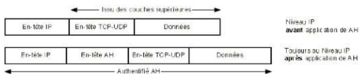
Figure 24.26 Authentification AH en mode Transport
