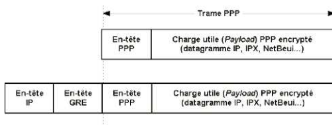
Figure 26.17 Trame PPTP
