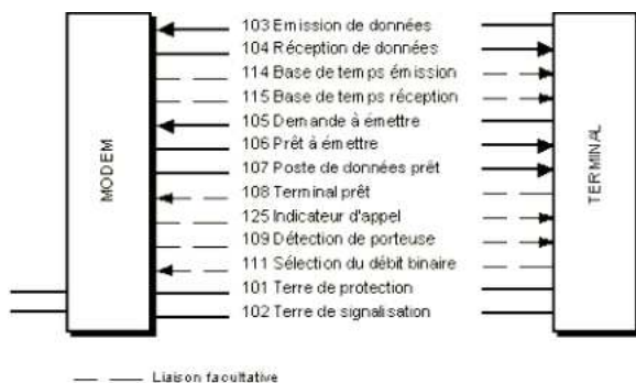
Figure 22.8 Connexion DB25
