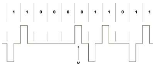
Figure 5.12 Encodage HDB3
