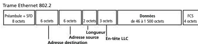
Figure 25.5 Trame Ethernet 802.2
