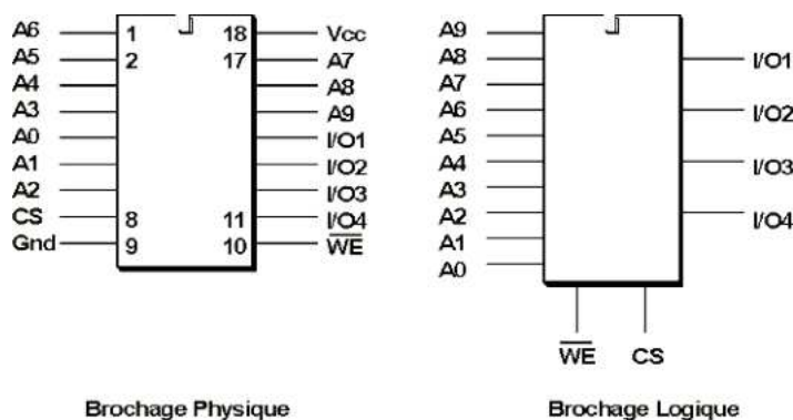
Figure 11.10 Brochage mémoire
