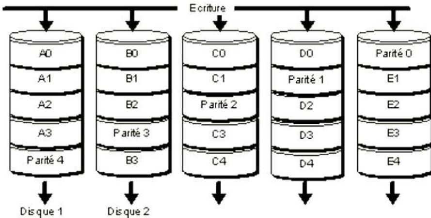
Figure 13.11 RAID 5
